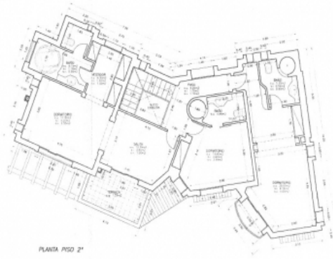
Floor plan
