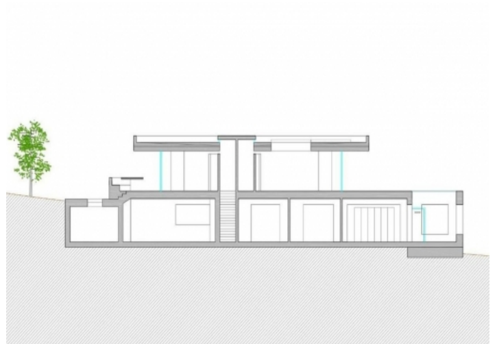
Construction plan
